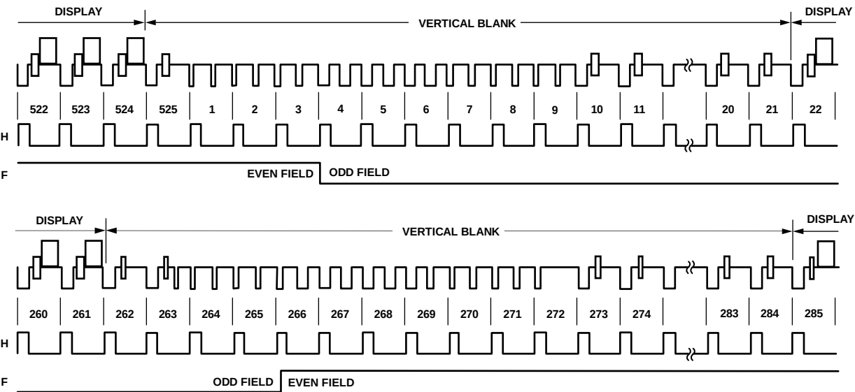
Figure 105. SD Timing Mode 0, Master Option, NTSC
