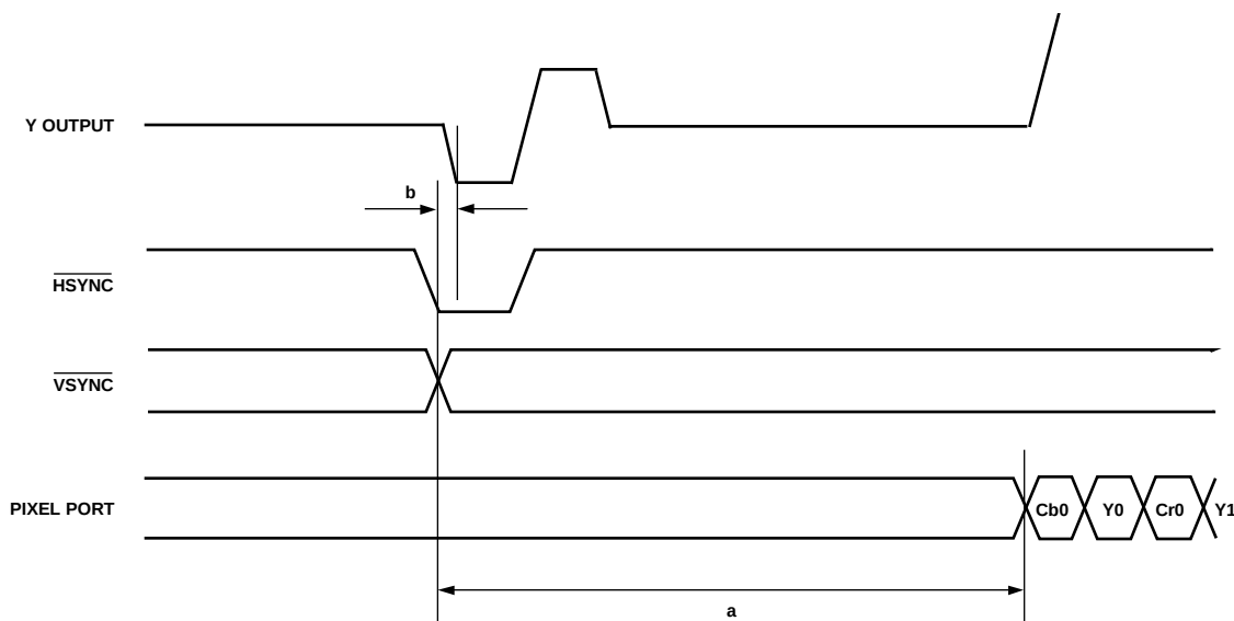
Figure 14. HD-SDR, 16-Bit 4:2:2 YCrCb ( \overline{\text{HSYNC}} / \overline{\text{VSYNC}} ) Input Timing Diagram
