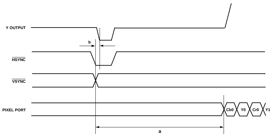
Figure 12. ED-SDR, 16-Bit 4:2:2 YCrCb ( \overline{\text{HSYNC}} / \overline{\text{VSYNC}} ) Input Timing Diagram
