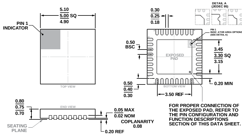
Figure 146. 32-Lead Lead Frame Chip Scale Package [LFCSP] 5 mm × 5 mm Body and 0.75 mm Package Height (CP-32-13)
