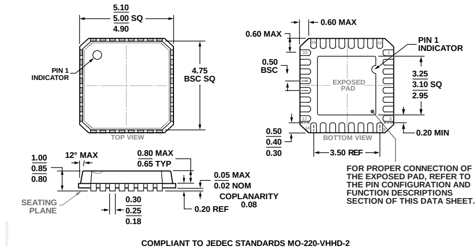
Figure 145. 32-Lead Lead Frame Chip Scale Package [LFCSP] 5 mm × 5 mm Body and 0.85 mm Package Height (CP-32-2)
