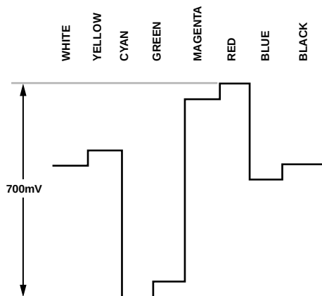
Figure 119. Pr Levels—NTSC
