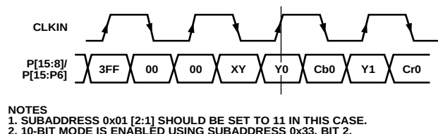
Figure 58. ED/HD-DDR Input Sequence (EAV/SAV)—Option B
