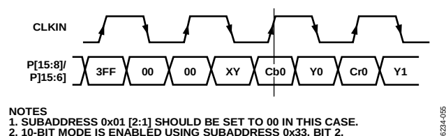
Figure 57. ED/HD-DDR Input Sequence (EAV/SAV)—Option A
