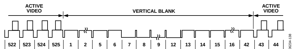
Figure 139. EAV/SAV Input Data Timing Diagram (SMPTE 293M)
