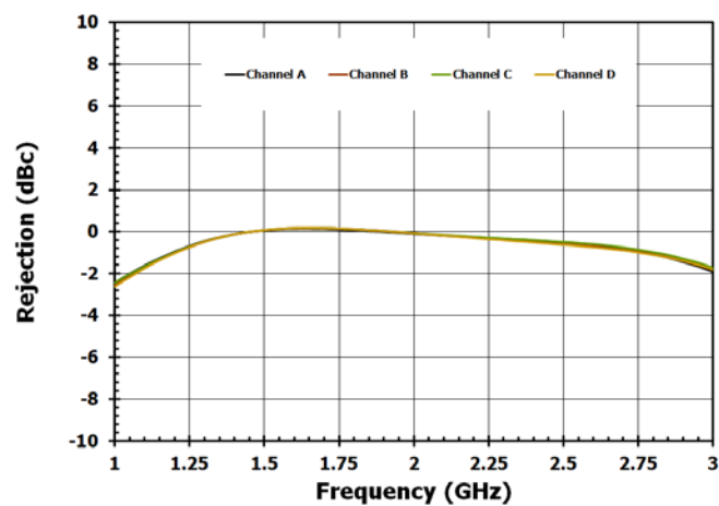
Figure 29. Out of Band Rejection vs Channel (w.r.t. 2.1GHz)
