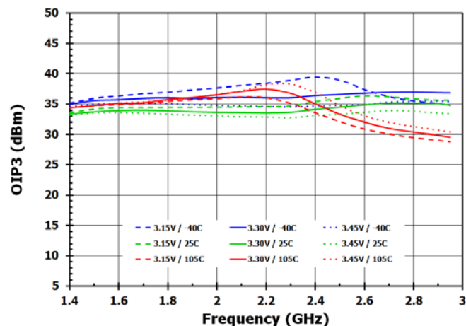
Figure 61. Band 2 OIP3 at DSA = 4dB
