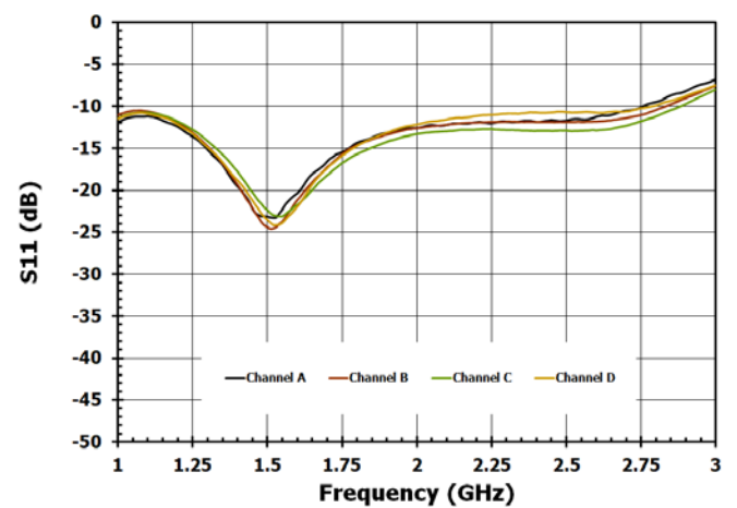
Figure 19. Input Return Loss vs Channel (DSA = 0dB)
