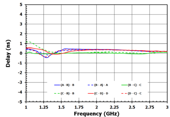
Figure 49. Cross Channel vs Channel Group Delay at DSA = 28dB
