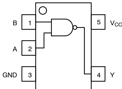
Figure 1. Pinout
