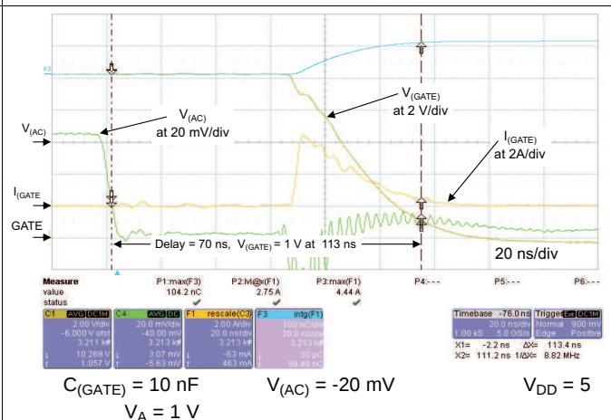
Figure 20. Turnoff Time
