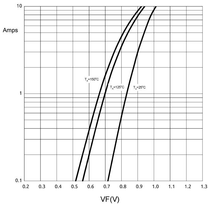
FIG3: Forward Voltage
