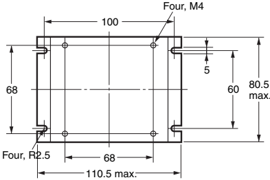
Mounting Holes
