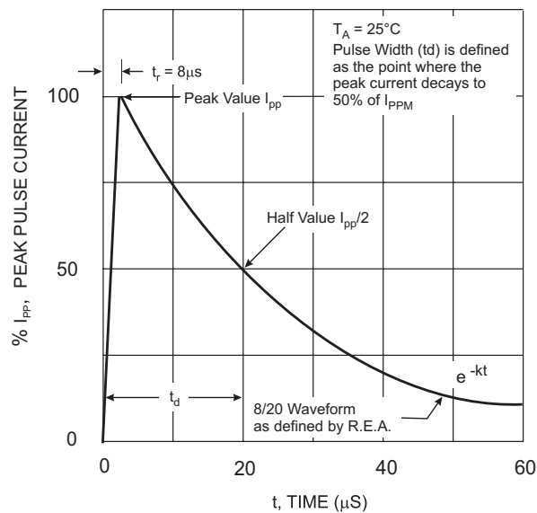
Fig. 3 Pulse Waveform
