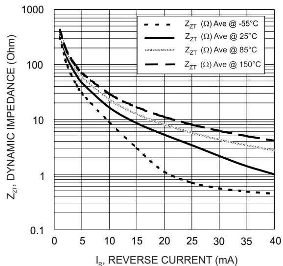
Fig. 11 Dynamic Impedance vs. Reverse Current (Small Signal)
