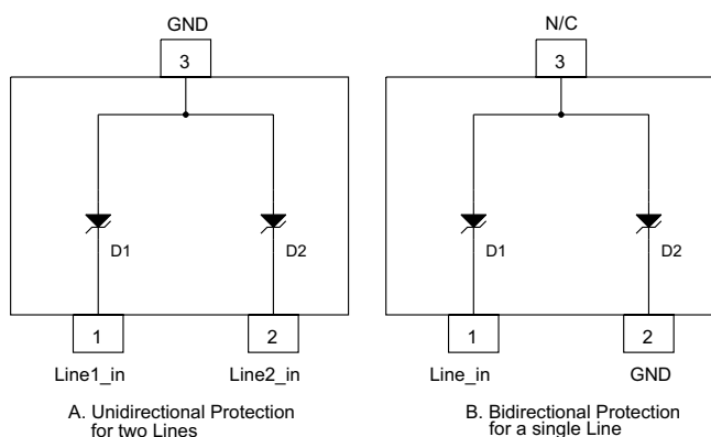
Fig. 1: Schematic and Pin Configuration
