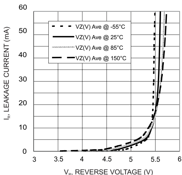
Fig. 9 Typical Reverse Characteristic
