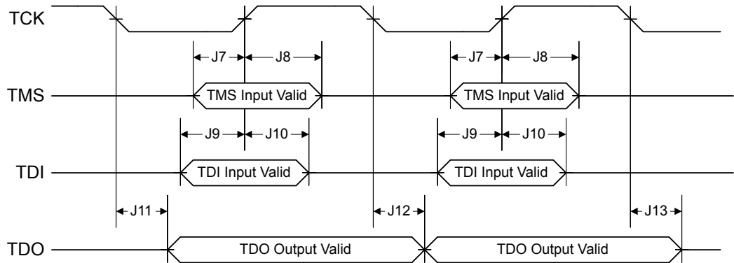
Figure 28-3. JTAG Test Access Port (TAP) Timing
