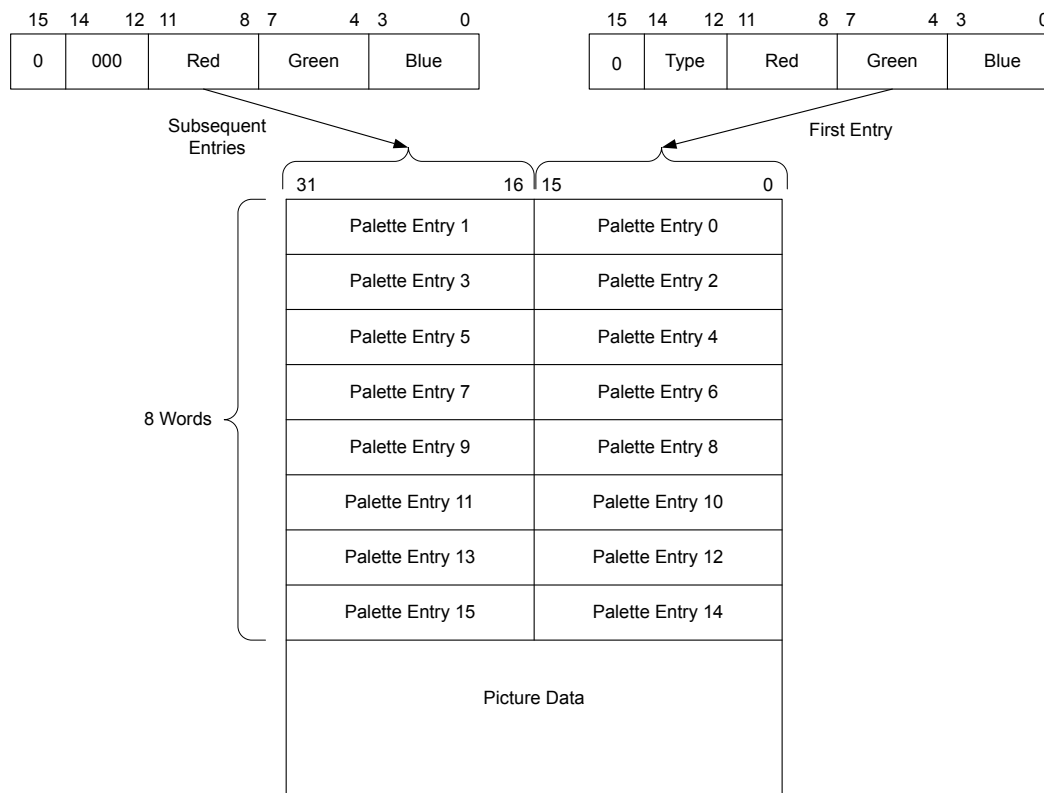
Figure 22-4. Palette RAM Structure for 1, 2, and 4 Bits Per Pixel
