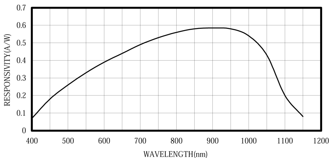
RESPONSIVITY
