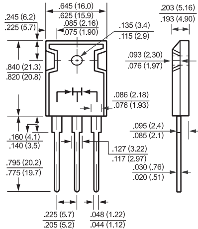
TO-3P
