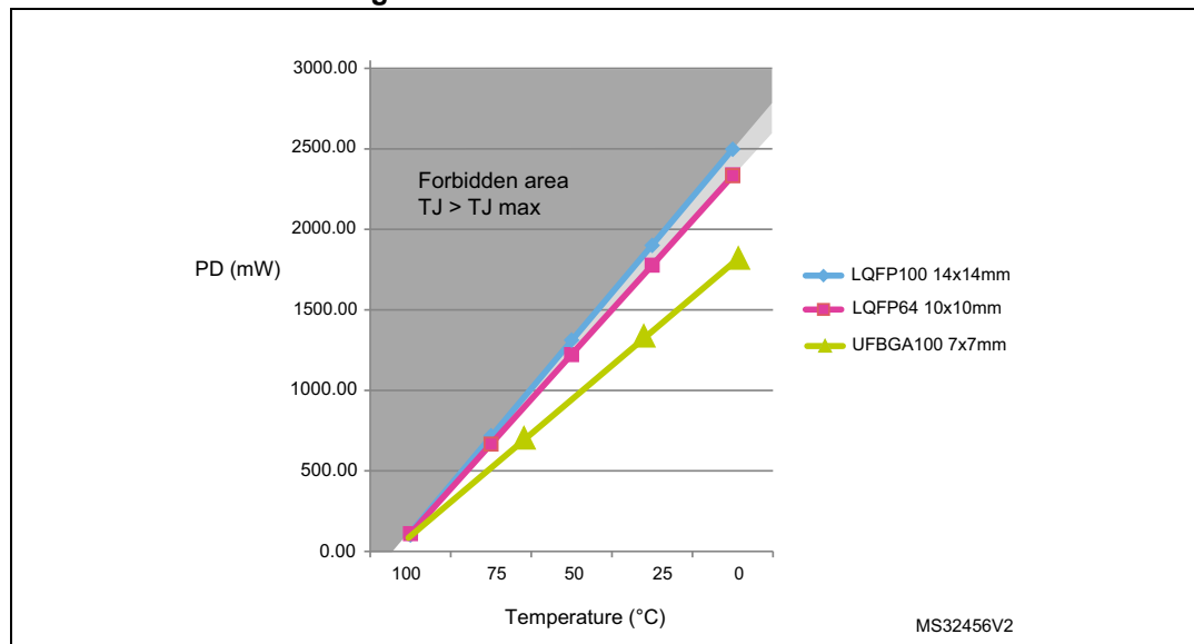
Figure 38. Thermal resistance suffix 6
