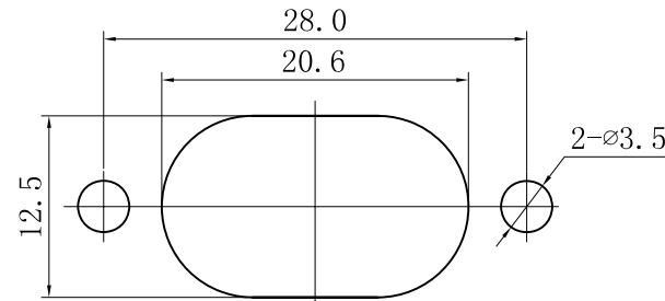
PANEL CUT-OUT
