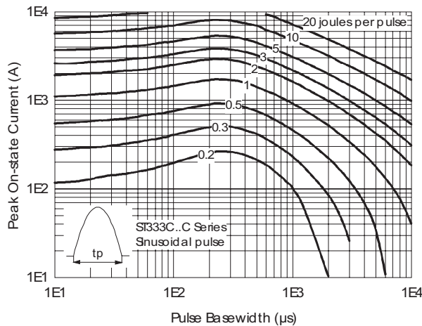
Fig. 16 - Maximum On-State Energy Power Loss Characteristics
