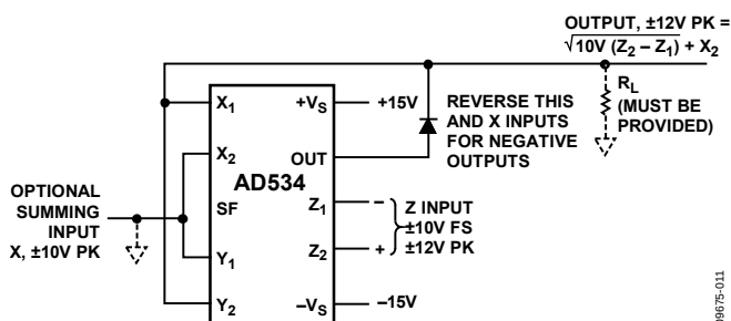
Figure 19. Square-Rooter Connection
