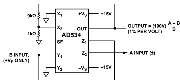
Figure 24. Percentage Computer
