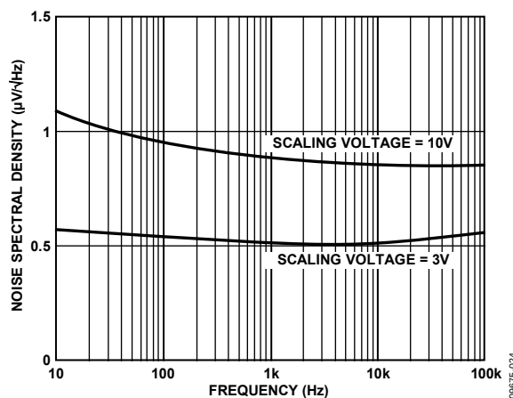
Figure 11. Noise Spectral Density vs. Frequency
