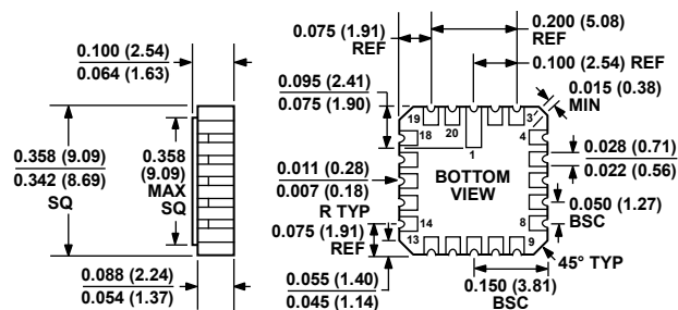
Figure 30. 20-Terminal Ceramic Leadless Chip Carrier [LCC] (E-20-1)
