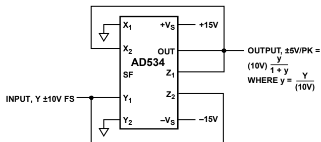
Figure 25. Bridge Linearization Function
