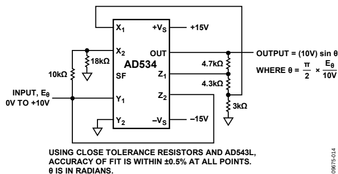
Figure 22. Sine Function Generator
