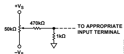
Figure 3. Optional Trimming Configuration
