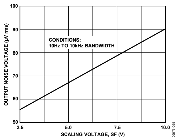
Figure 12. Wideband Noise vs. Scaling Voltage
