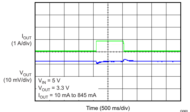
LOAD TRANSIENT
