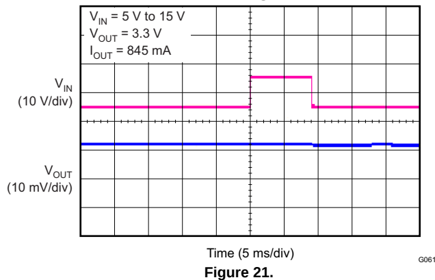
LINE TRANSIENT
