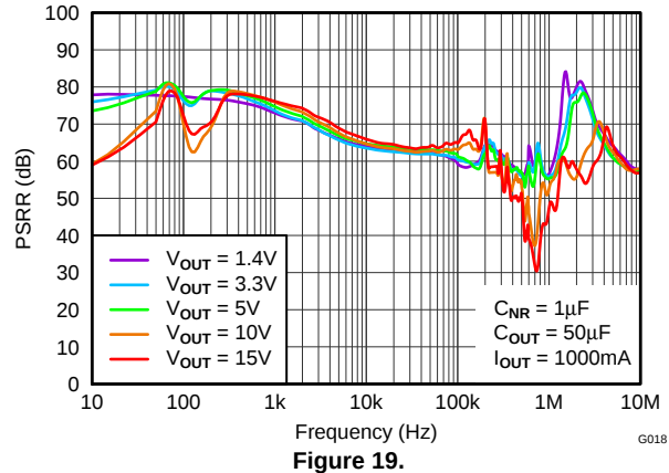
POWER-SUPPLY REJECTION RATIO vs OUTPUT VOLTAGE
