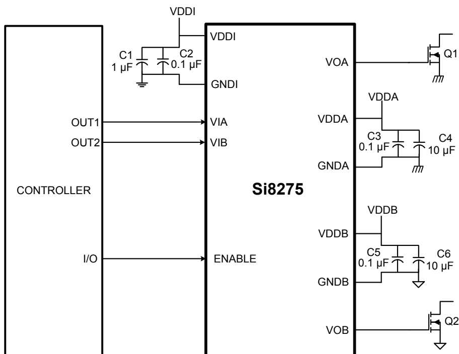
Figure 3.2. Si827x in a Dual Driver Application
