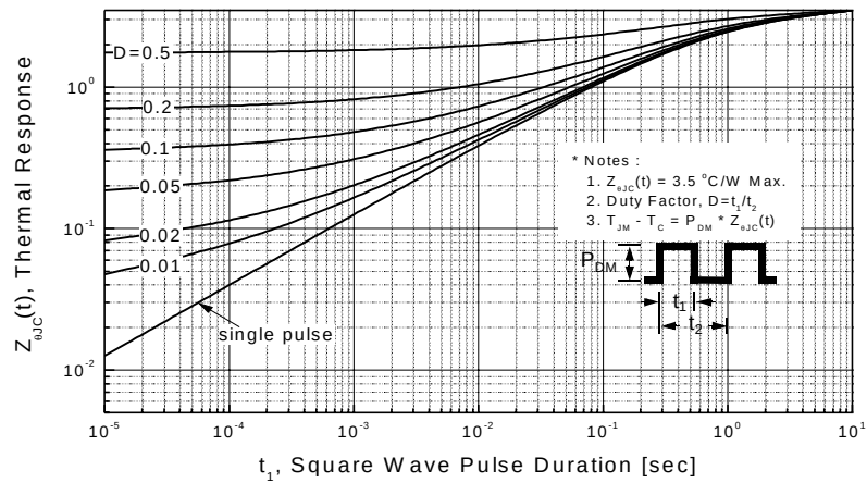
Figure 11-2. Transient Thermal Response Curve for FCPF11N60
