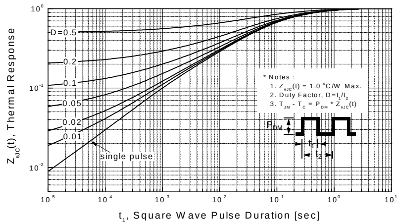
Figure 11-1. Transient Thermal Response Curve for FCP11N60
