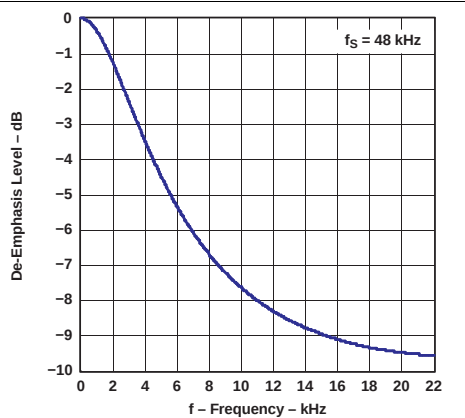
Figure 10. De-Emphasis
