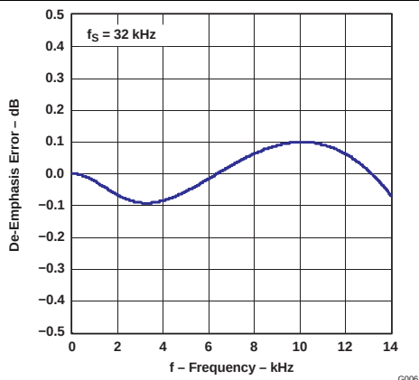
Figure 7. De-Emphasis Error
