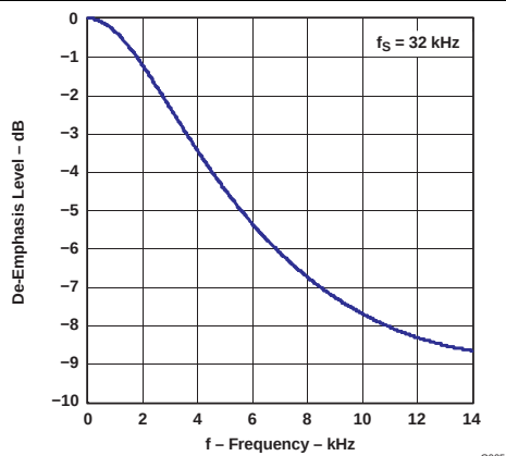
Figure 6. De-Emphasis
