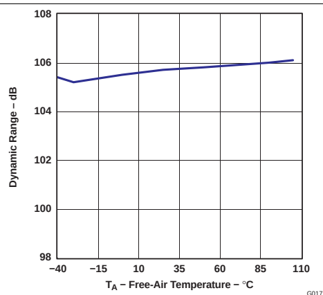
Figure 18. Dynamic Range vs Temperature
