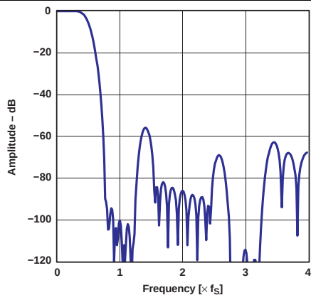
Figure 4. Frequency Response (Slow Roll-off)
