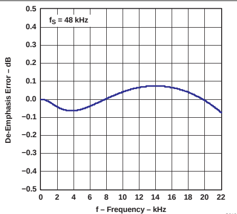
Figure 11. De-Emphasis Error
