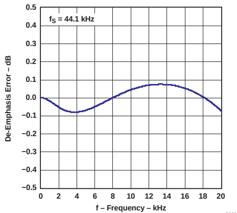
Figure 9. De-Emphasis Error
