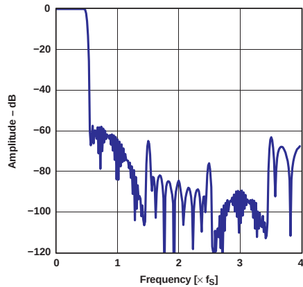
Figure 2. Frequency Response (Sharp Roll-off)
