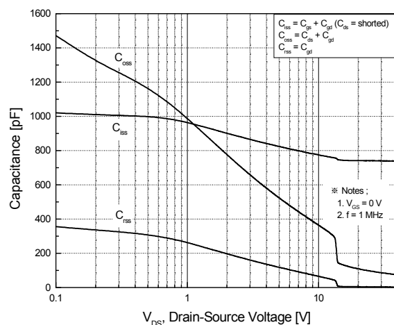
Fig.8 Capacitance Characteristics
