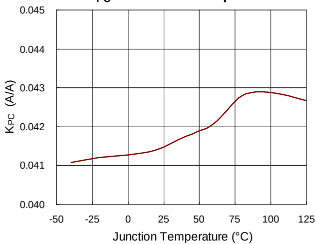
K_{PC} vs. Junction Temperature
