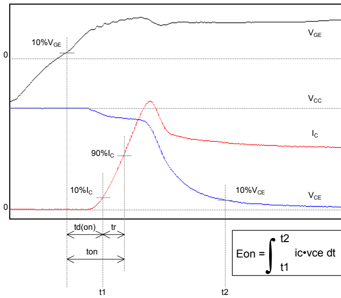
Fig. 3 – Definitions of switching times & energies of IGBT part
