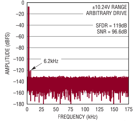
32k Point Arbitrary Two-Tone FFT f_{SAMPL} = 350\text{ksps} , IN^+ = -7\text{dBFS} 2kHz Sine, IN^- = -7\text{dBFS} 3.1kHz Sine
