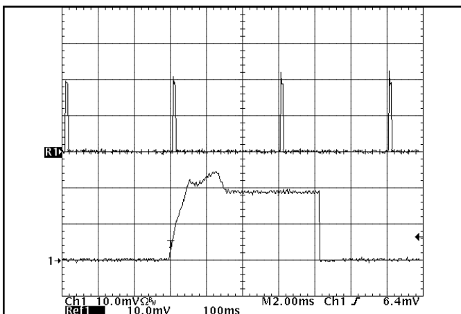
Figure 29: Load current for 1.225V output (10A/div) as a function of time when the converter attempts to turn on into a 10 m\Omega short circuit. Bottom trace is an expansion of the on-time portion of the top trace.
