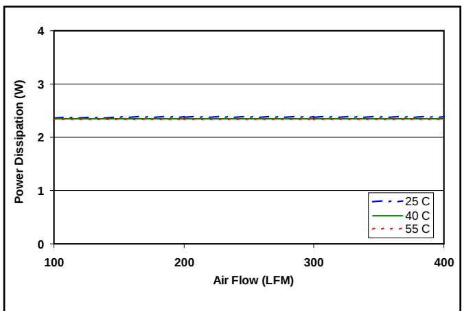
Figure 6: Power dissipation at 60% load and 50/50 power split (4.5A load on 1.225V and 2.5A load on 2.45V) versus air flow rate for ambient air temperatures of 25°C, 40°C, and 55°C (nominal input voltage).
