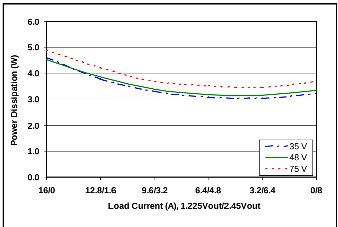
Figure 4: Power dissipation vs. load current, with total output power fixed at 100% (20W) and load current split as shown between 1.225V and 2.45V outputs at minimum, nominal, and maximum input voltage at 25°C.
