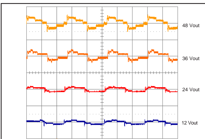
Figure 11: Output voltage response for 12 V, 24 V, 36 V, and 48 Vout to step-change in load current (50-75-50% of Iout max; di/dt=0.1A/ \mu s). Load cap: 100 \mu F, 100m \Omega ESR tant, Vout (2 V/div).
