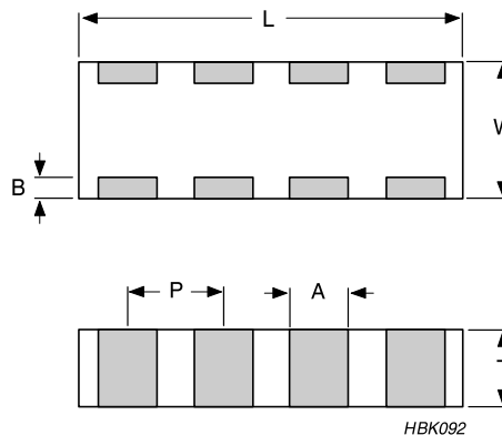
Fig. 3 Surface mounted multilayer ceramic capacitor dimension
