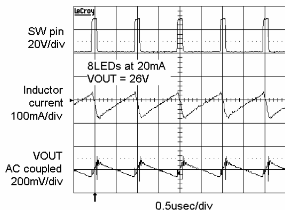
Switching Waveforms
