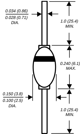
DO-204AP
