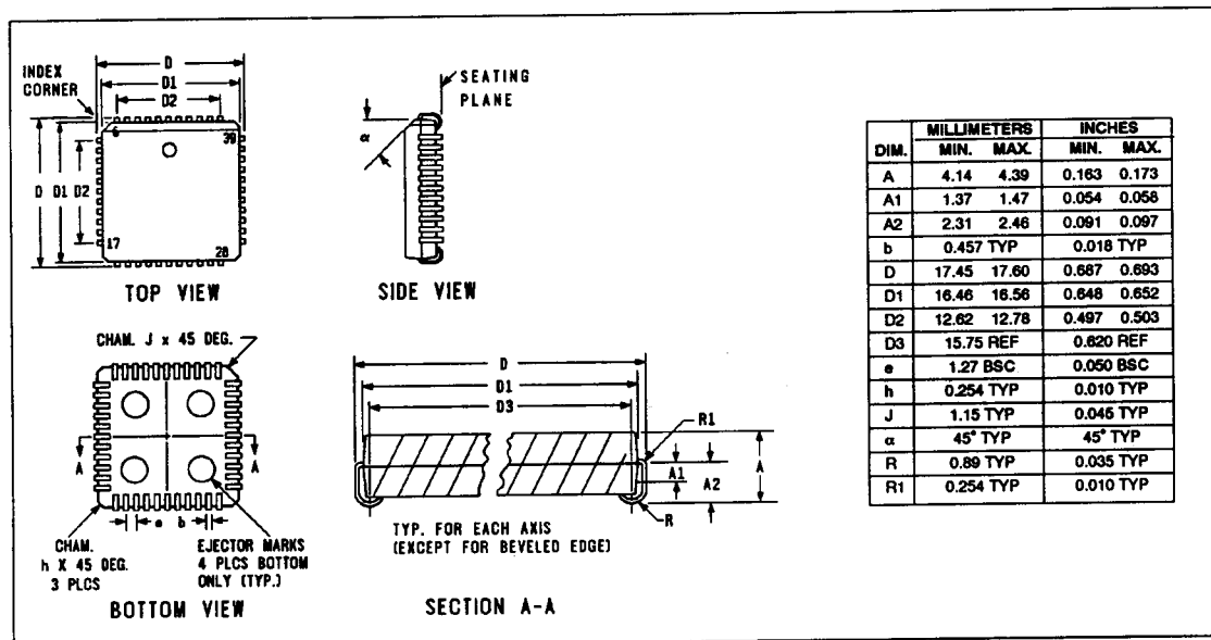
44-Pin PLCC
