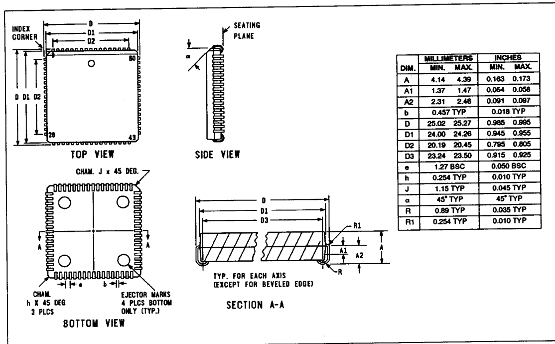
68-Pin PLCC
