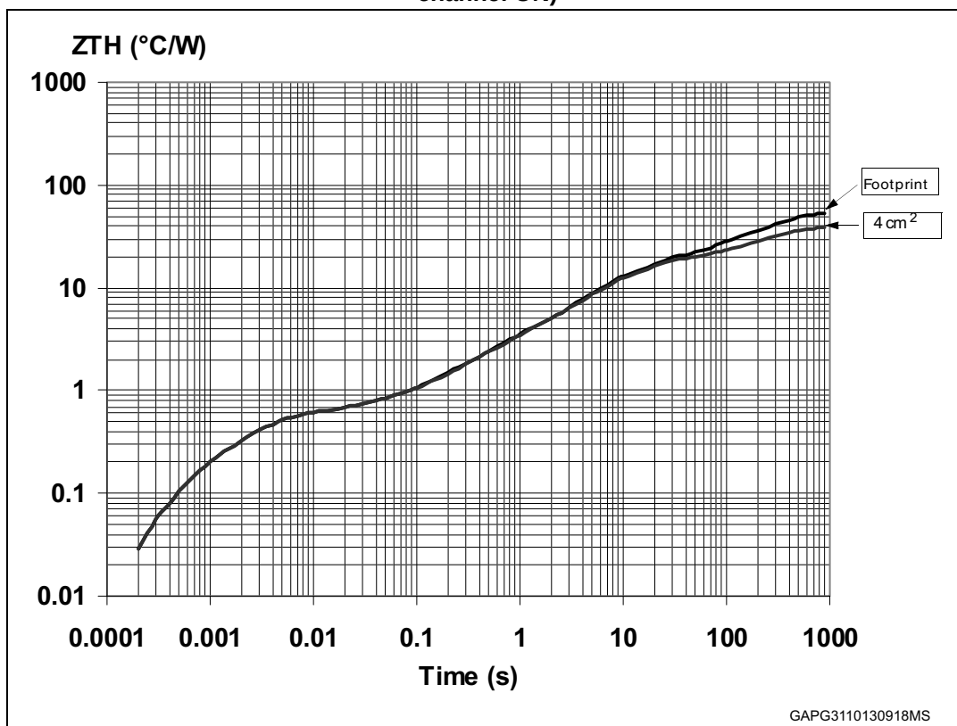
Figure 26. MultiPowerSO-30 thermal impedance junction ambient single pulse (one channel ON)
