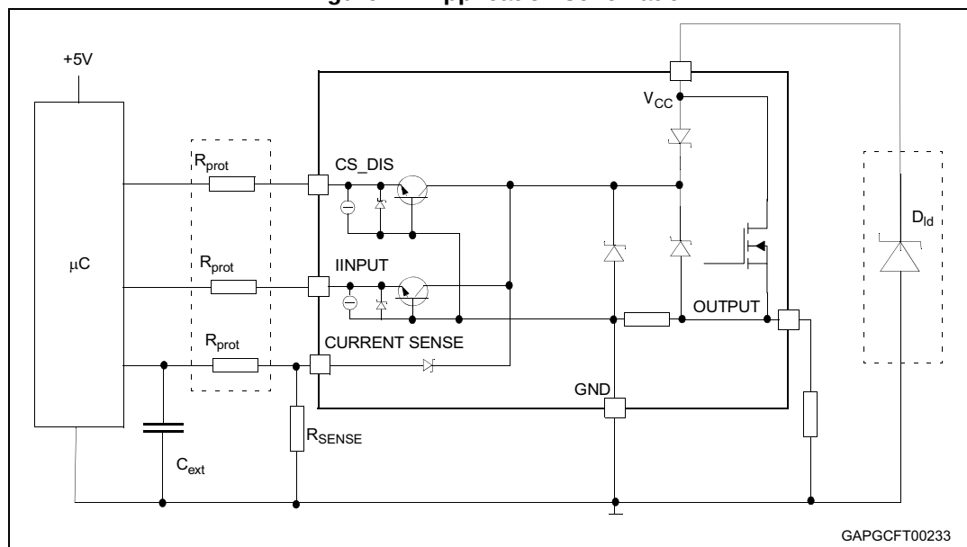
Figure 22. Application schematic
