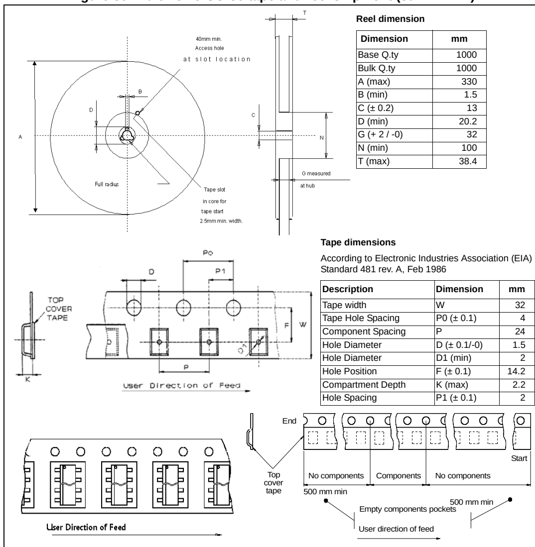
Figure 30. MultiPowerSO-30 tape and reel shipment (suffix "TR")
