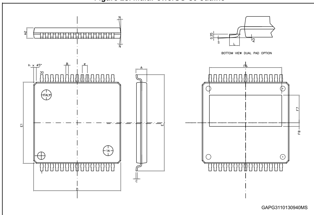
Figure 28. MultiPowerSO-30 outline
