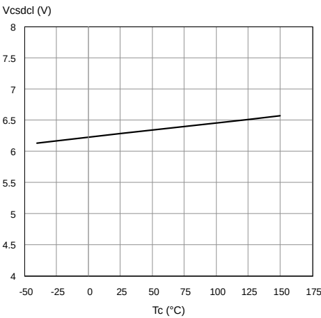
Figure 20. CS_DIS clamp voltage
