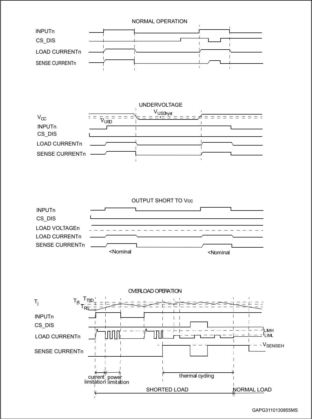
Figure 6. Waveforms
