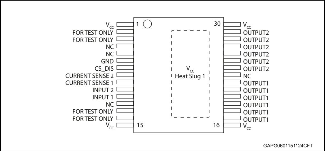
Figure 2. Configuration diagram (not in scale)
