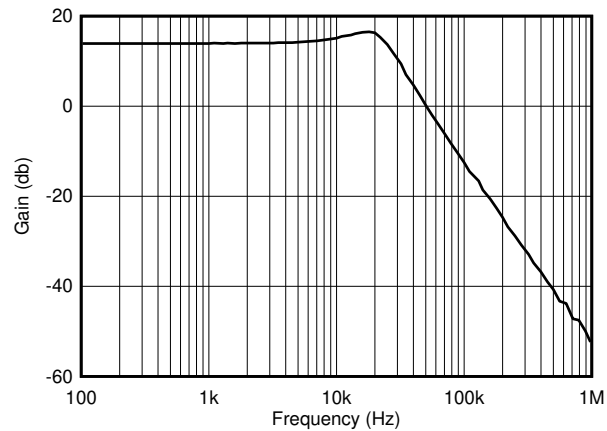
Figure 48. OPAx202 Second-Order, 25-kHz, Chebyshev, Low-Pass Filter
