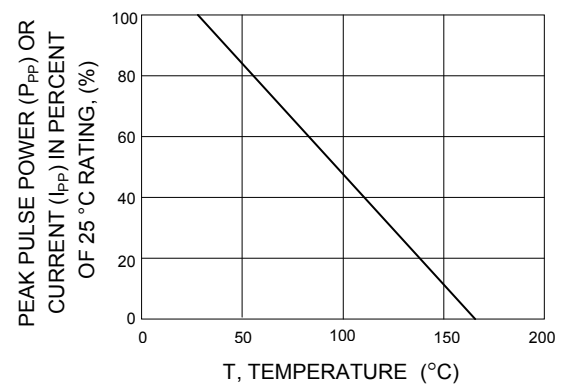
FIG.2 - DERATING CURVE
