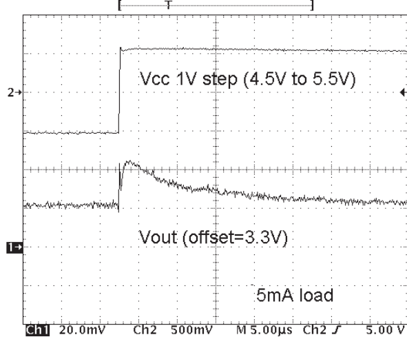
Fig 2.15 V_{CC} Load Step Response Rising
