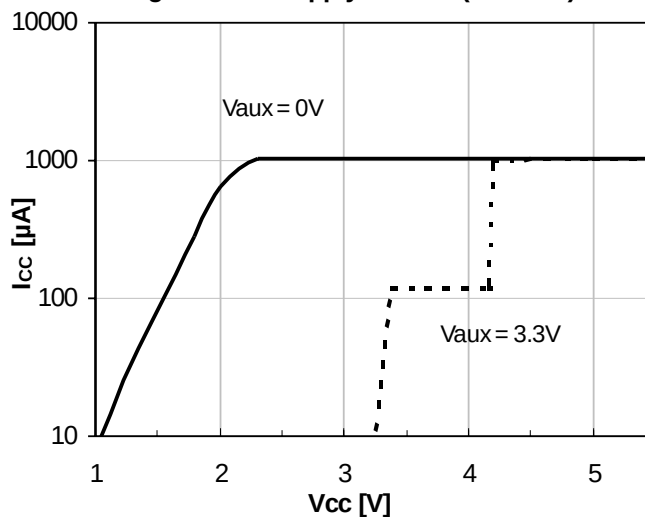
Fig 1.5. Vcc Supply Current (No Load)
