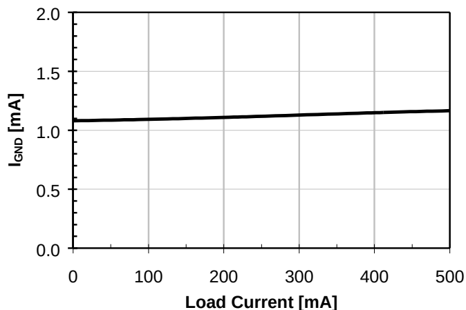
Fig 1.4. Ground Current
