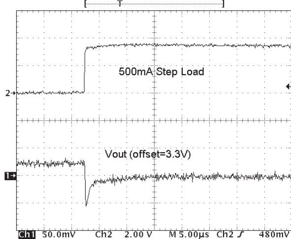
Fig 2.13 V_{CC} Load Transient Response Rising
