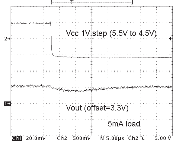
Fig 2.16 V_{CC} Load Step Response Falling
