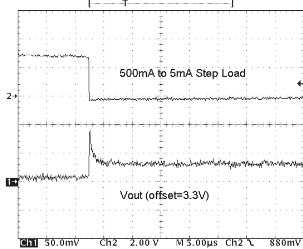
Fig 2.14 V_{CC} Load Transient Response Falling
