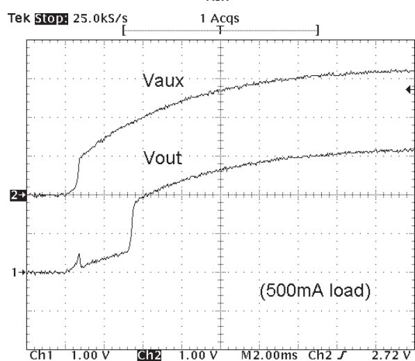
Fig 2.5 V_{AUX} cold start
