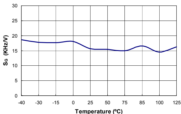
Figure 14. Green-Mode-Frequency Decreasing Rate (S G ) vs. Temperature
