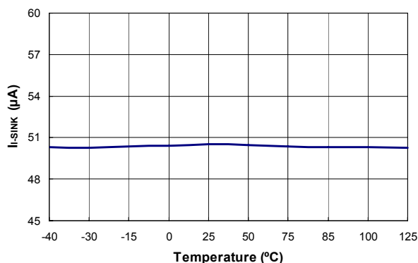
Figure 20. Output Sink Current ( I_{i-SINK} ) vs. Temperature
