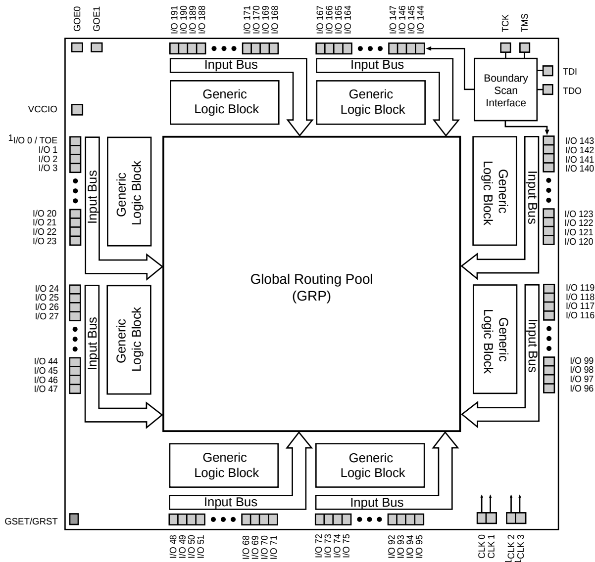
Figure 1. ispLSI 5256V Functional Block Diagram (272 BGA Option)
