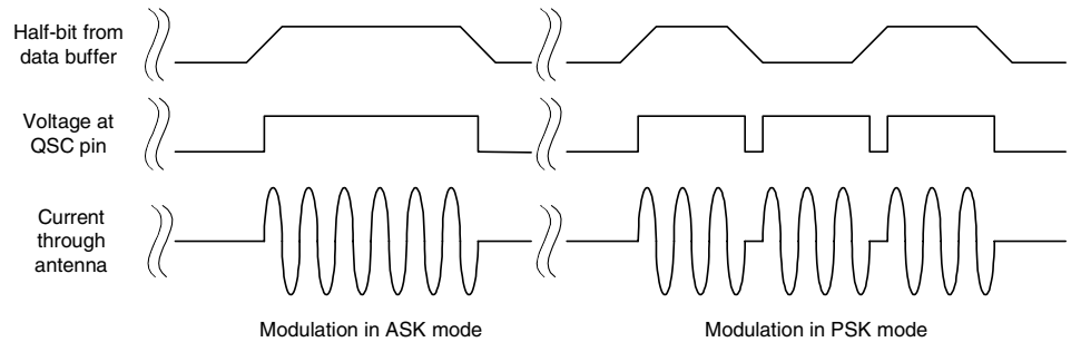
Figure 13. QSC Operation
