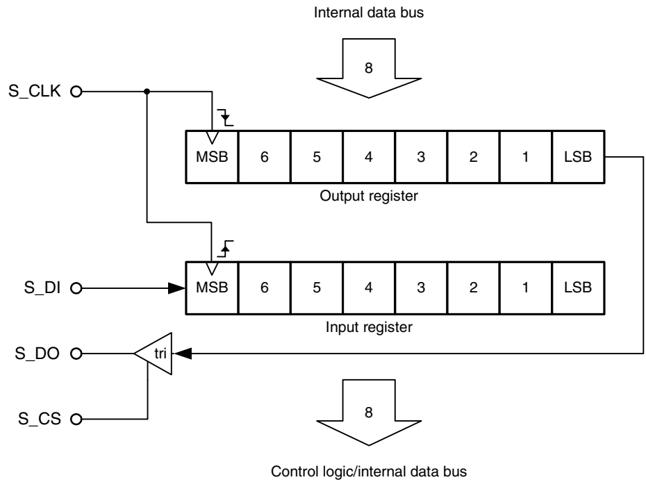
Figure 8. SPI Structure
