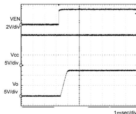
Fig.5 Input sequence 2
