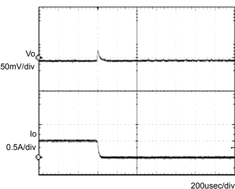
Fig.2 Transient Response
