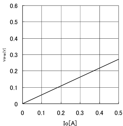
Fig.22 Minimum dropout Voltage 4 ( V_{cc}=8\text{V} , T_a=25^\circ\text{C} )
