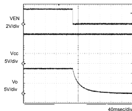
Fig.6 OFF sequence 2
