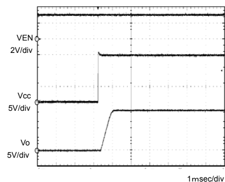
Fig.3 Input sequence 1
