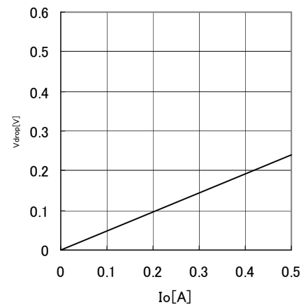
Fig.23 Minimum dropout Voltage 5 ( V_{cc}=10\text{V} , T_a=25^\circ\text{C} )
