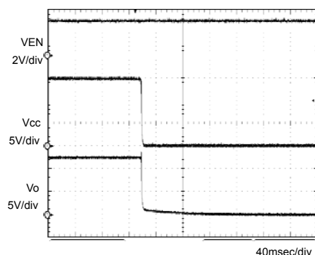
Fig.4 OFF sequence 1
