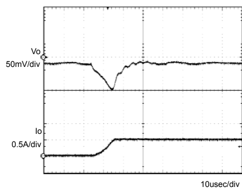
Fig.1 Transient Response
