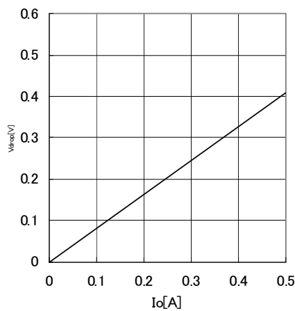
Fig.20 Minimum dropout Voltage 2 ( V_{cc}=4.5\text{V} , T_a=25^\circ\text{C} )
