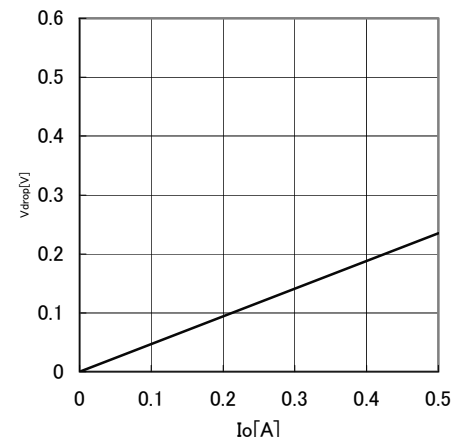
Fig.24 Minimum dropout Voltage 6 ( V_{cc}=12\text{V} , T_a=25^\circ\text{C} )
