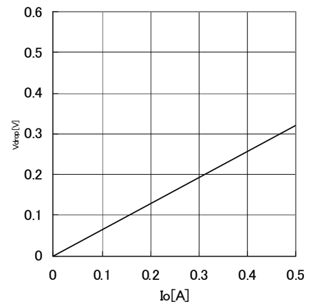
Fig.21 Minimum dropout Voltage 3 ( V_{cc}=6\text{V} , T_a=25^\circ\text{C} )
