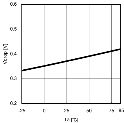
Fig.16 Minimum dropout Voltage 1 ( V_{cc}=5\text{V} , I_o=-0.5\text{A} )
