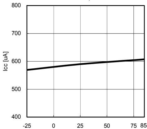
Fig.8 T_a - I_{CC}
