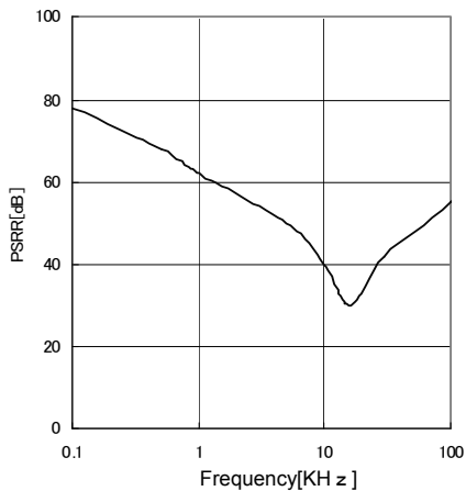
Fig.19 PSRR ( I_o=0\text{mA} )
