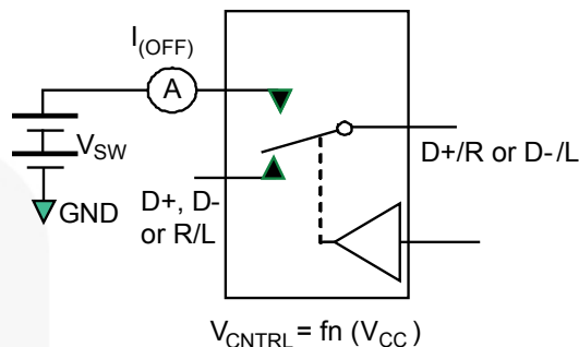
Figure 5. Off Leakage
