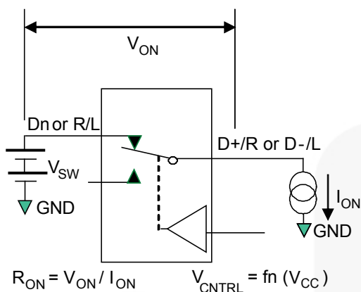
Figure 4. On Resistance
