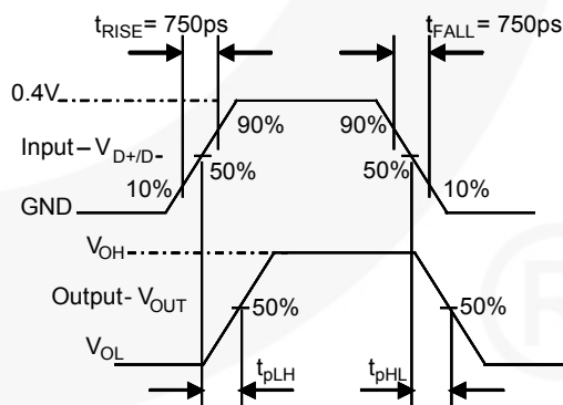
Figure 9. USB Switch Propagation Delay Waveforms
