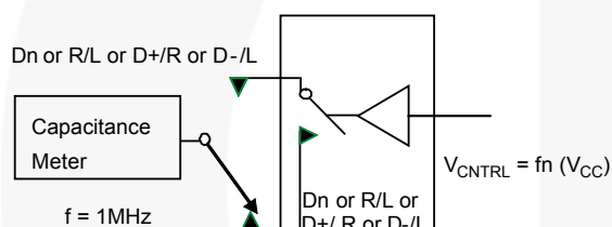
Figure 12. Channel Off Capacitance
