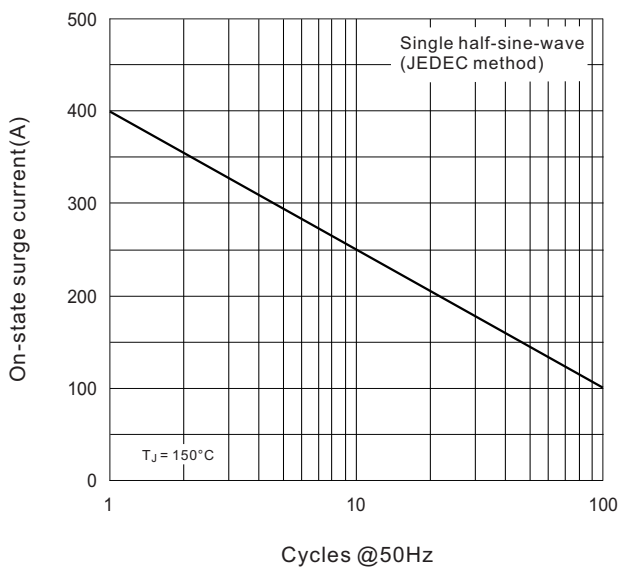
Fig.3 On-state surge current vs. cycles
