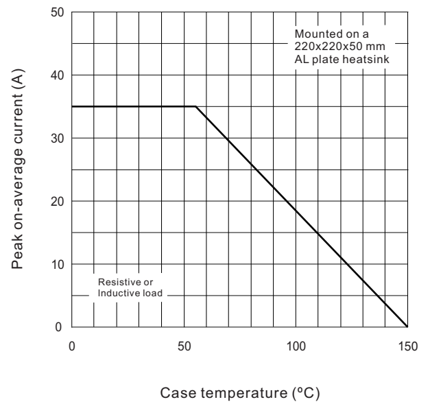
Fig.2 Case temperature vs on-state average current
