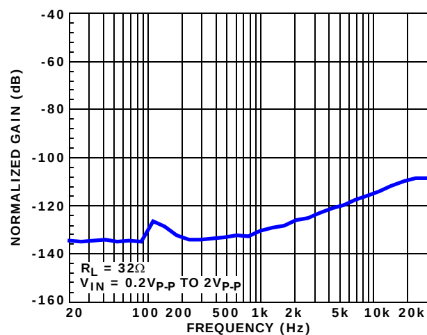
FIGURE 13. OFF-ISOLATION
