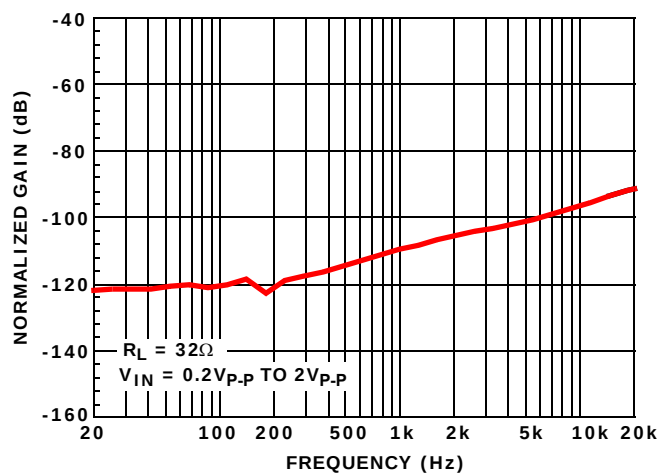
FIGURE 14. CROSSTALK
