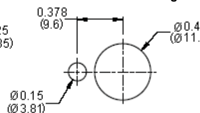
15/32 In Bushing
