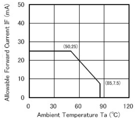
Ambient Temp. vs Allowable Forward Current:
