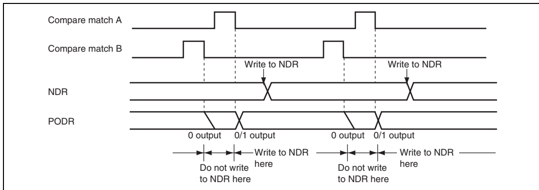
Figure 11.7 Non-Overlapping Operation and NDR Write Timing
