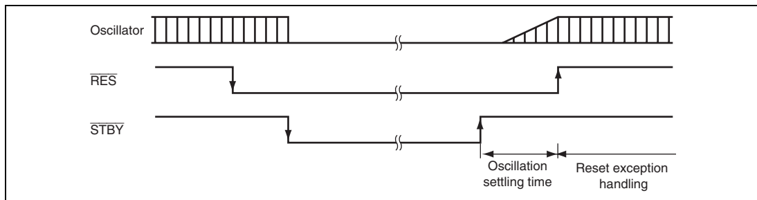
Figure 20.3 Hardware Standby Mode Timing
