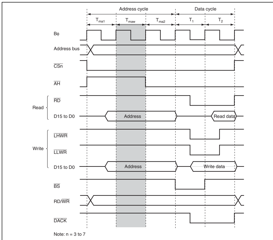
Figure 6.32 Access Timing of 3 Address Cycles (ADDEX = 1)
