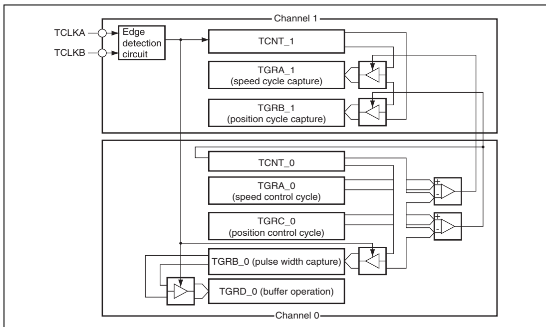
Figure 10.29 Phase Counting Mode Application Example
