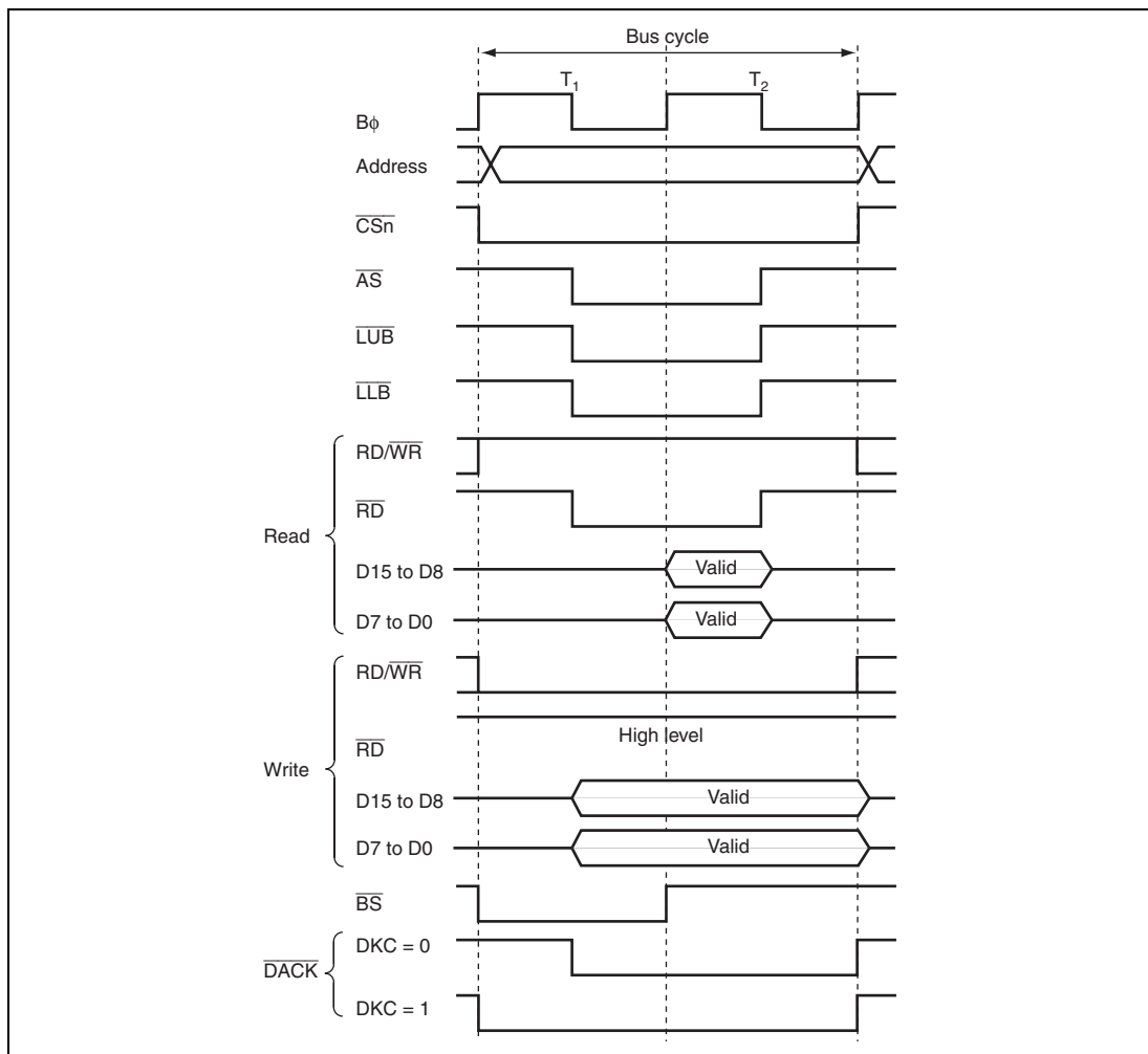
Figure 6.27 \overline{\text{DACK}} Signal Output Timing
