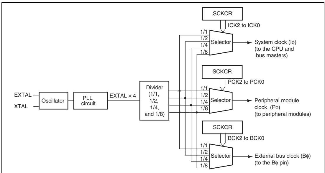
Figure 19.1 Block Diagram of Clock Pulse Generator
