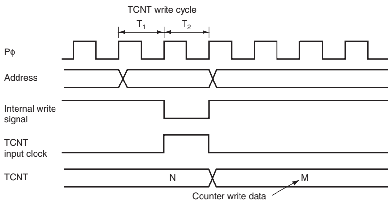
Figure 13.5 Conflict between TCNT Write and Increment
