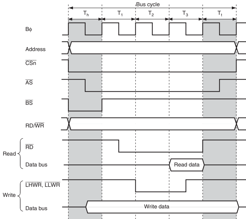
Figure 6.3 \overline{CS} and Address Assertion Period Extension (Example of Basic Bus Interface, 3-State Access Space, and RDNn = 0)
