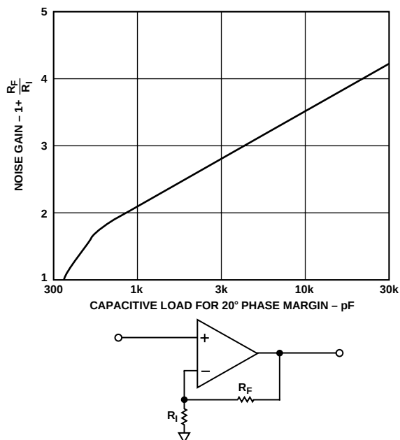
Figure 41. Capacitive Load Tolerance vs. Noise Gain
