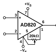
Figure 43. Offset Null
