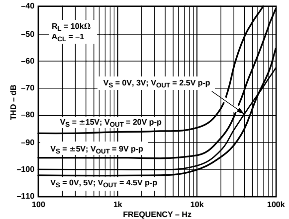
Figure 14. Total Harmonic Distortion vs. Frequency
