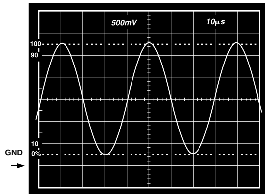
Figure 37. V_S = 3\text{ V} , 0\text{ V} ; Gain of Two Inverter, V_{IN} = 1.25\text{ V} , 25 kHz, Sine Wave Centered at -0.75\text{ V} , R_L = 600\text{ Ω}
