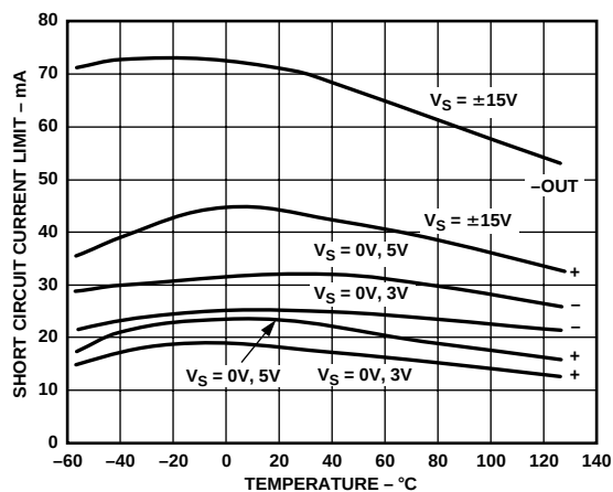
Figure 22. Short Circuit Current Limit vs. Temperature
