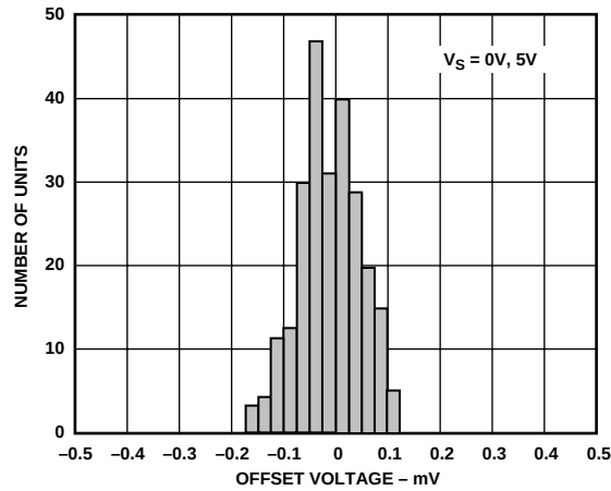
Figure 3. Typical Distribution of Offset Voltage (248 Units)
