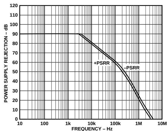
Figure 24. Power Supply Rejection vs. Frequency
