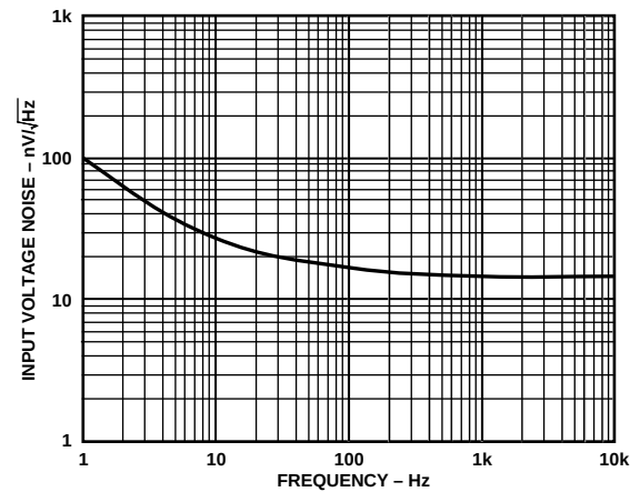
Figure 13. Input Voltage Noise vs. Frequency
