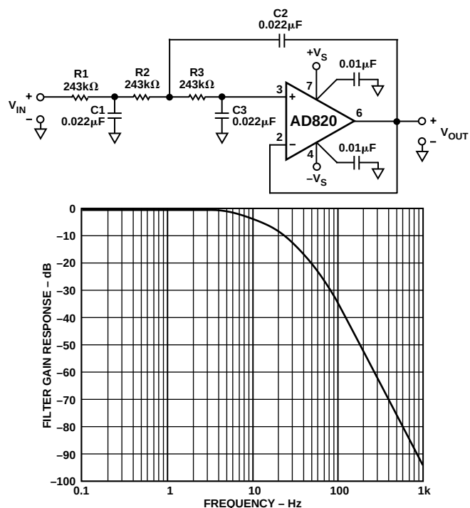
Figure 46. 10 Hz Sallen Key Low-Pass Filter
