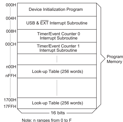
Program Memory
