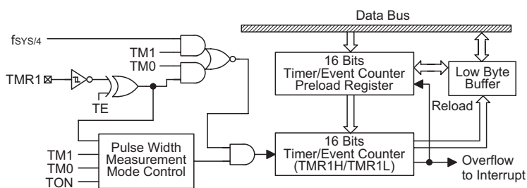
Timer/Event Counter 1
