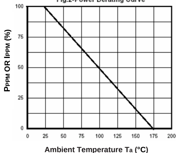
Fig.2-Power Derating Curve
