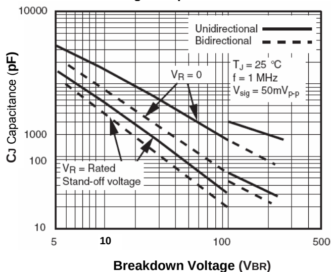
Fig.6- Capacitance
