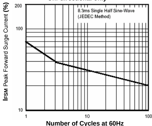
Fig.4- Max. Non-Repetitive Forward Surge Current Uni-directional only
