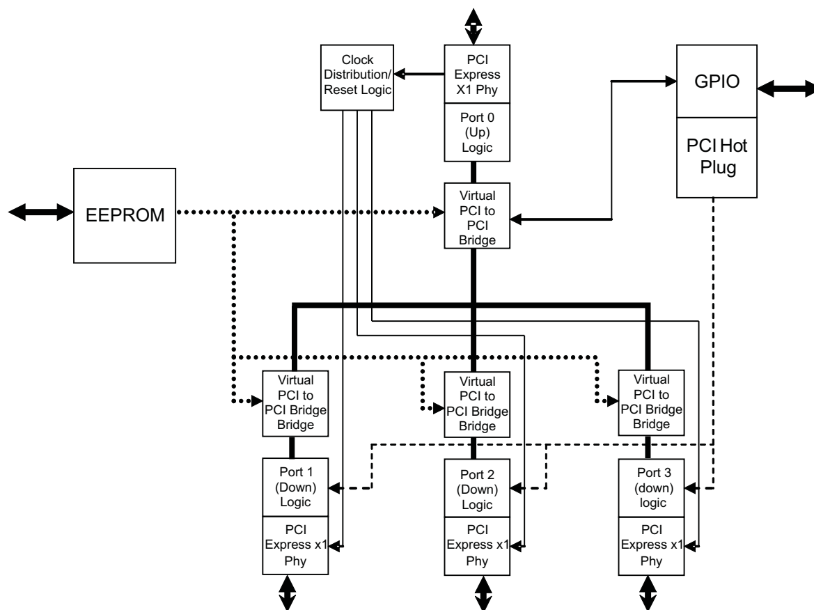
Figure 3-1. Block Diagram
