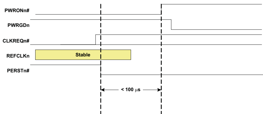
Figure 5-4. Normal Power-Down
