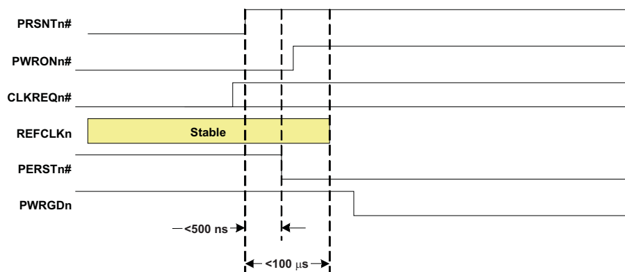
Figure 5-5. Surprise Removal
