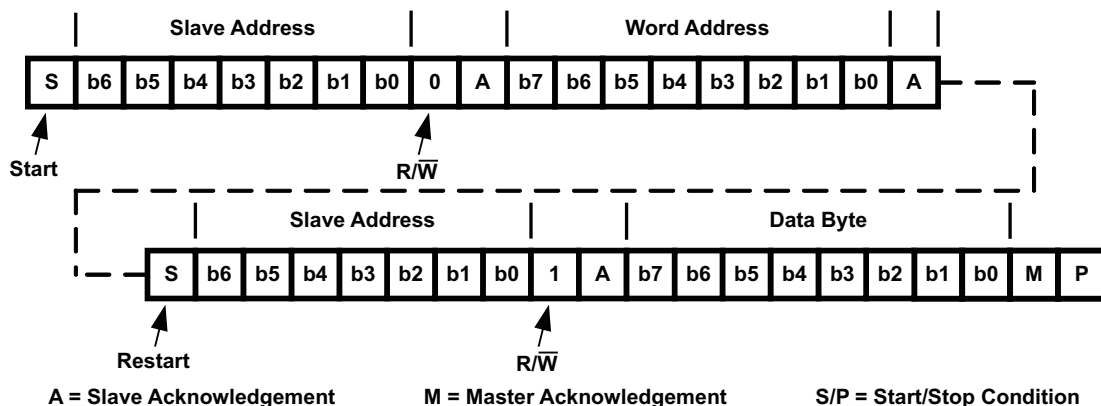
Figure 3-8. Serial-Bus Protocol – Byte Read
