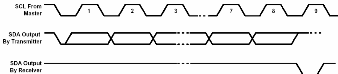
Figure 3-6. Serial-Bus Protocol Acknowledge
