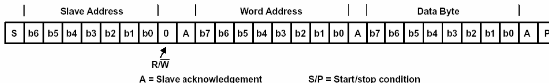
Figure 3-7. Serial-Bus Protocol – Byte Write
