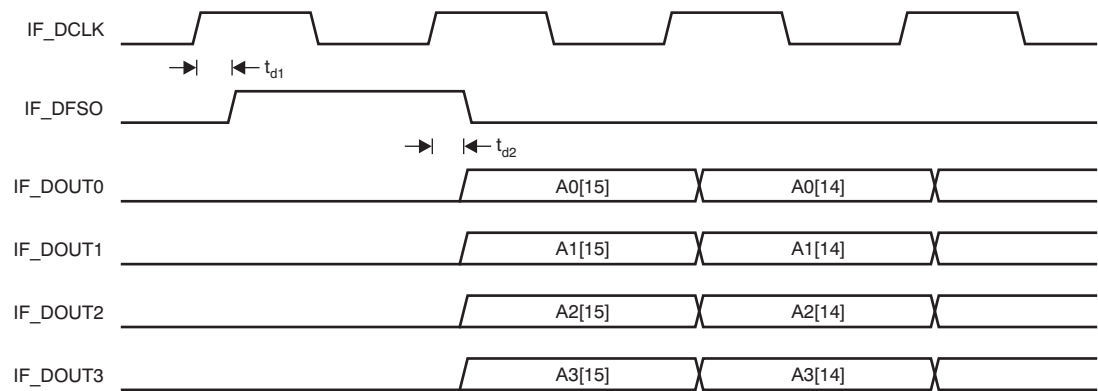
Figure 16. Detailed Timing
