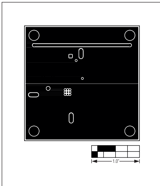
Figure 8. MAX15101/MAX15102/MAX15103 EV Kits PCB Layout—Solder Side
