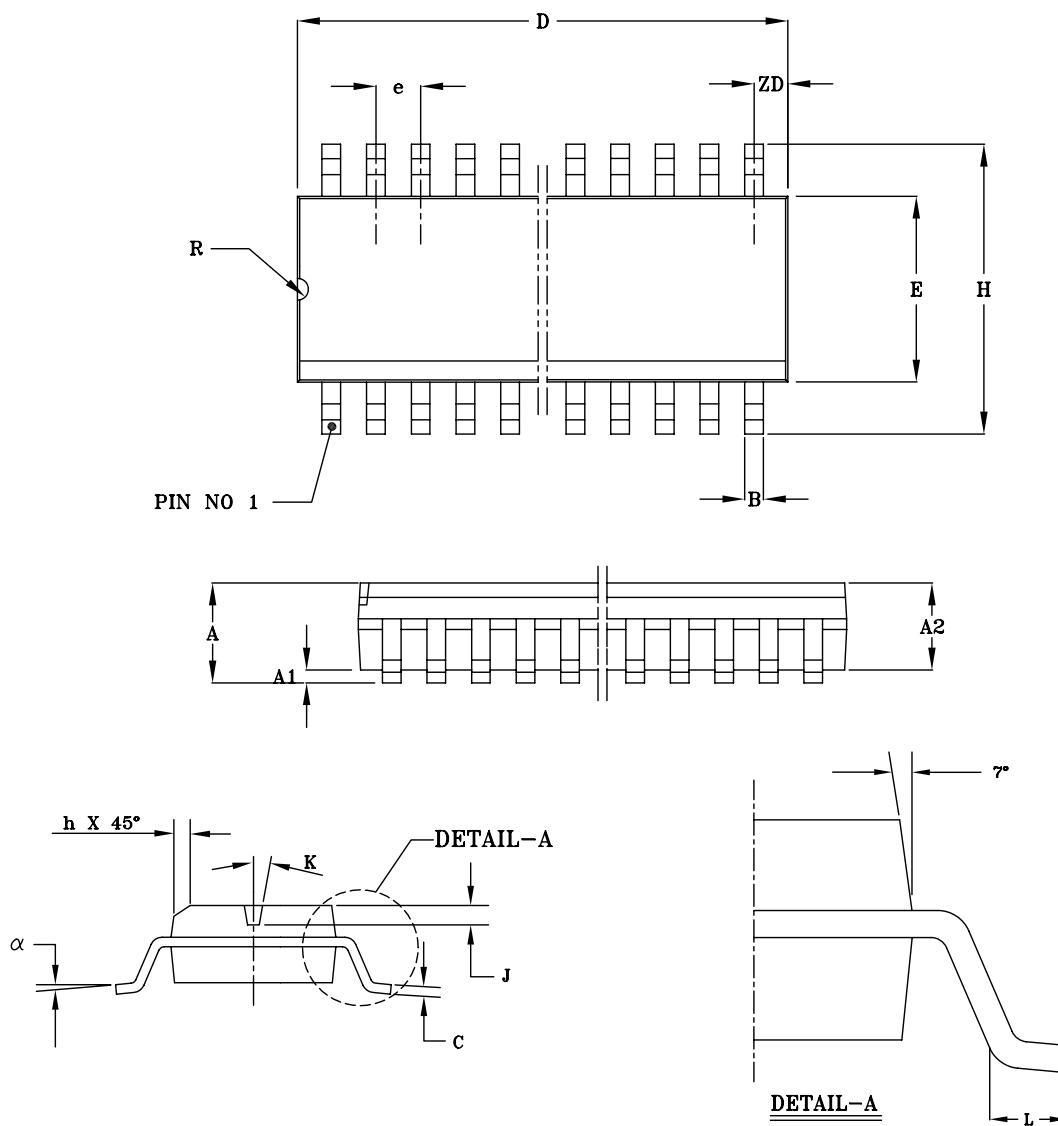
Figure 16. 24-pin SOIC Package
