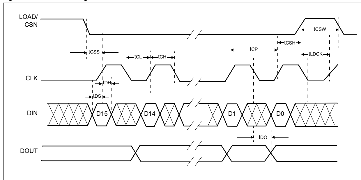
Figure 11. Interface Timing
