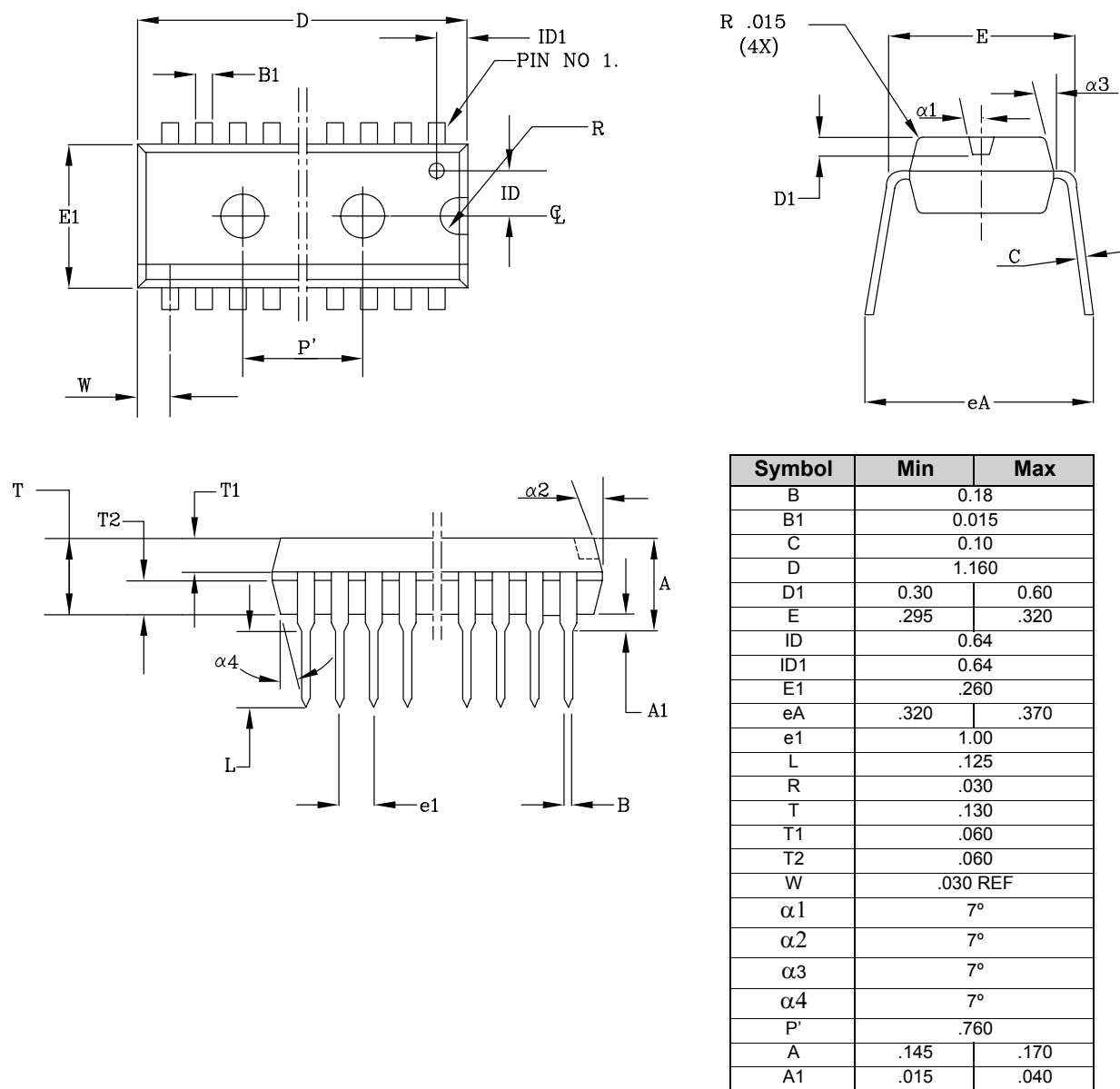
Figure 15. 24-pin DIP Package
