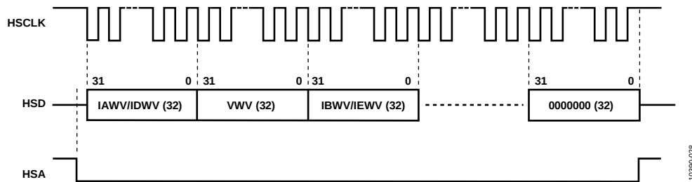
Figure 44. HSDC Communication for HGAP = 0, HXFER[1:0] = 01, and HSAPOLE = 0; HSIZE Is Irrelevant
