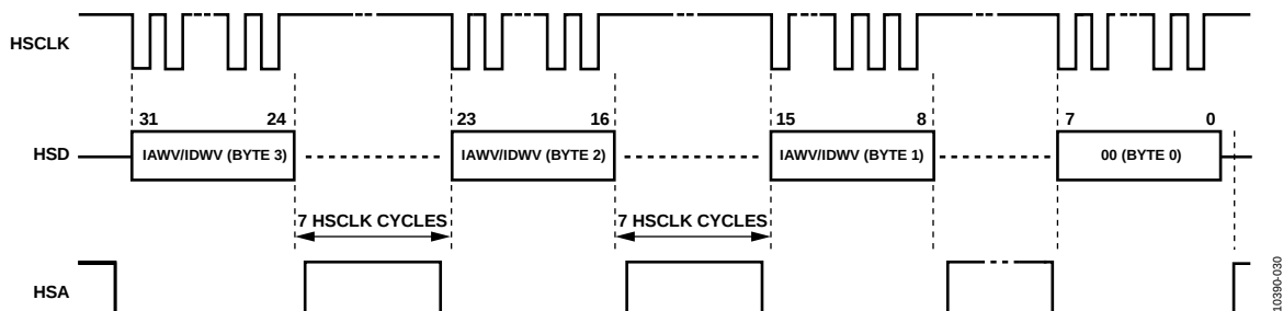
Figure 46. HSDC Communication for HSIZE = 1, HGAP = 1, HXFER[1:0] = 01, and HSAPOLE = 0
