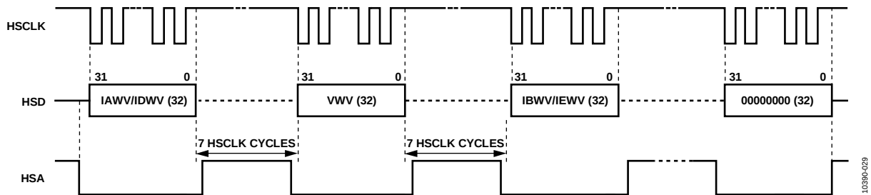
Figure 45. HSDC Communication for HSIZE = 0, HGAP = 1, HXFER[1:0] = 01, and HSAPOLE = 0
